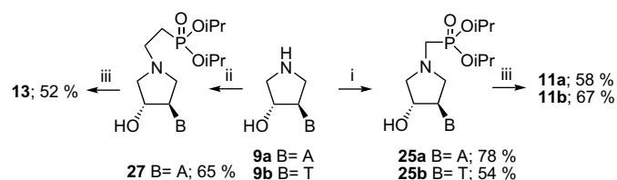
Scheme 4. Synthesis of trans -nucleotide analogues from pyrrolidine nucleosides. (i) HP(O)(O i Pr) 2 , formaldehyde; (ii) diisopropyl vinylphosphonate, CH 3 OH; (iii) Me 3 SiBr, DMF (MeCN).
