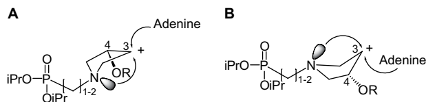
Figure 3. Possible explanation of C3 epimerization during nucleophilic displacement.
