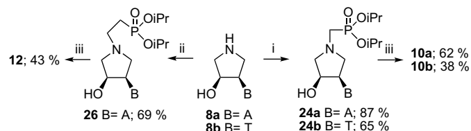
Scheme 3. Synthesis of cis -nucleotide analogues from pyrrolidine nucleosides. (i) HP(O)(O i Pr) 2 , formaldehyde; (ii) diisopropyl vinylphosphonate, CH 3 OH; (iii) Me 3 SiBr, DMF (MeCN).
