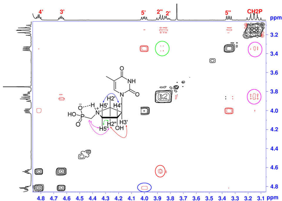
Figure 5. Part of H,H-ROESY spectrum of 11b at pD \sim 7 showing spatial arrangement in zwitterionic form.
