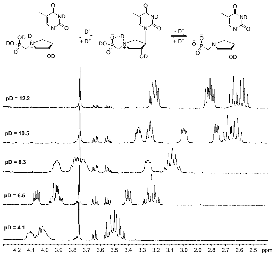
Figure 4. ^1\text{H} NMR spectra of 11b measured at different pD values.
