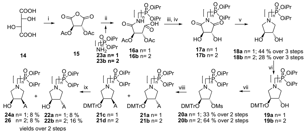
Scheme 2. Synthesis of pyrrolidine N -alkylphosphonate derivatives. (i) AcCl, reflux; (ii) 23a or 23b , DCM; (iii) Ac 2 O, 90 °C; (iv) 1 M HCl in MeOH; (v) NaBH 4 /I 2 /THF, aq HCl; (vi) DMTrCl/pyridine; (vii) MsCl/DMAP/DCM; (viii) Adenine/Cs 2 CO 3 /DMF; (ix) 80% aq AcOH.
